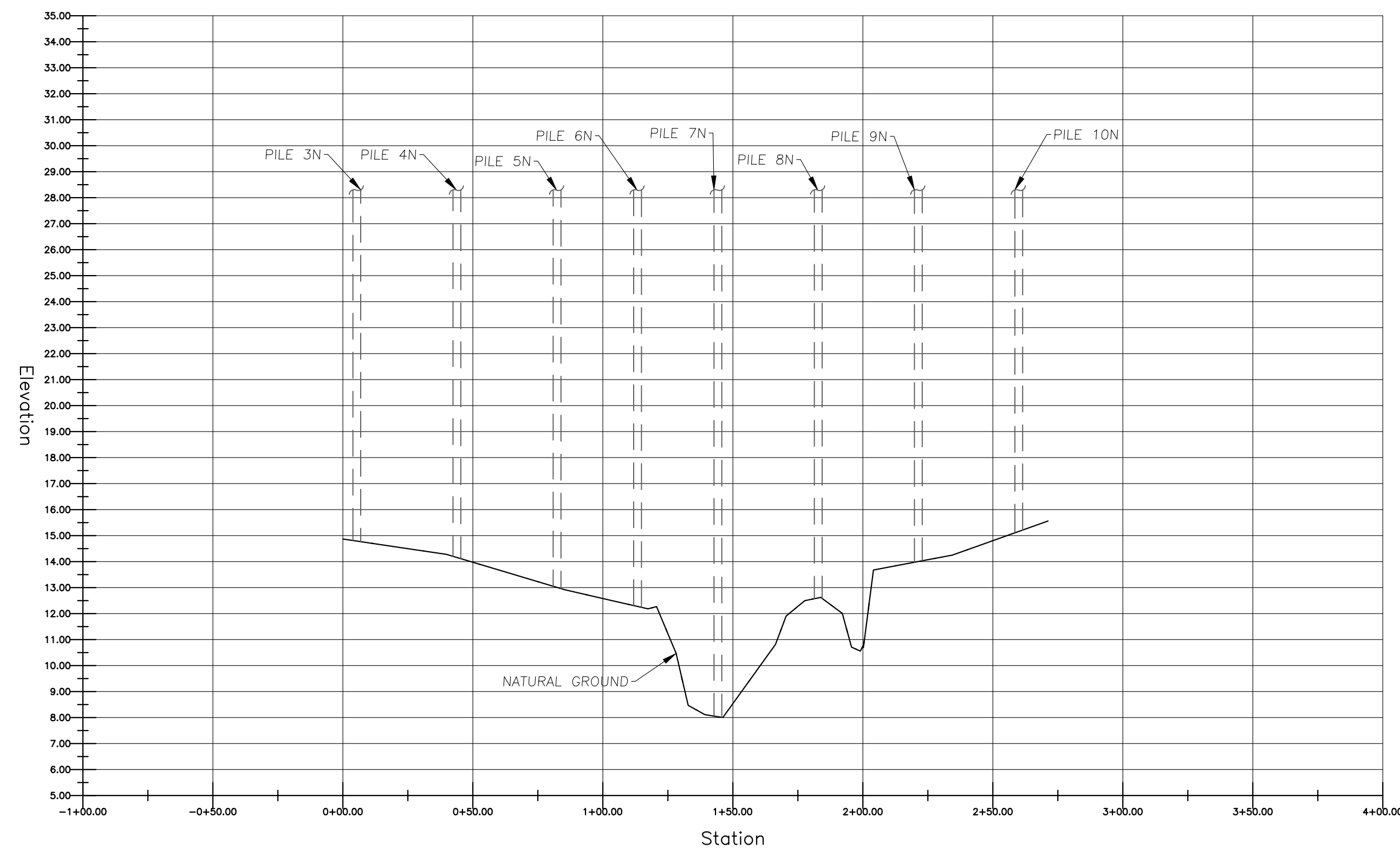
CROSS-SECTION (NORTH OF BRIDGE)
